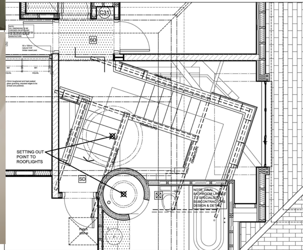
● LOFT PLAN
